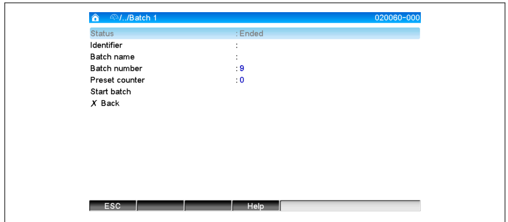
8 Batch menu
