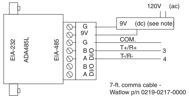
Figure 18b — CMC Non-Isolated Converter - ADA485L CMC Connecticut Micro-Computer, Inc., 1-800-426-2872, http://www.2cmc.com/
