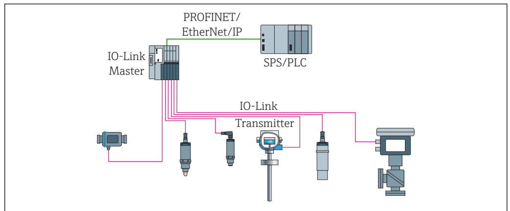
2 Temperature transmitter with IO-Link interface
